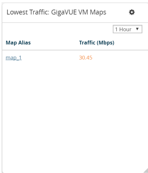
Figure 5 Lowest Traffic
