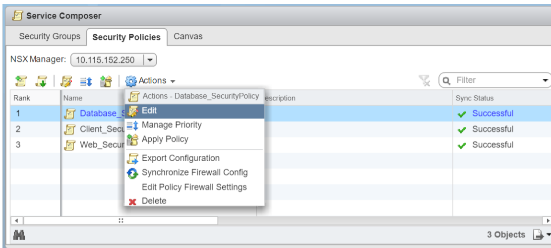
Figure 13 Edit Policy
