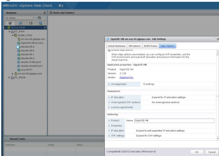
Figure 12 vApp Options
