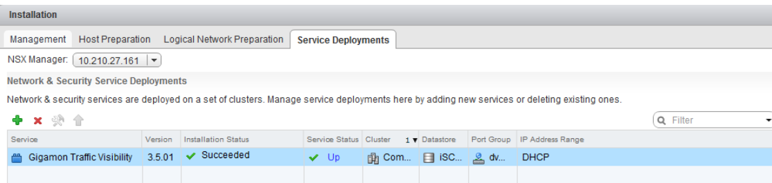
Figure 12 Update Succeeded
