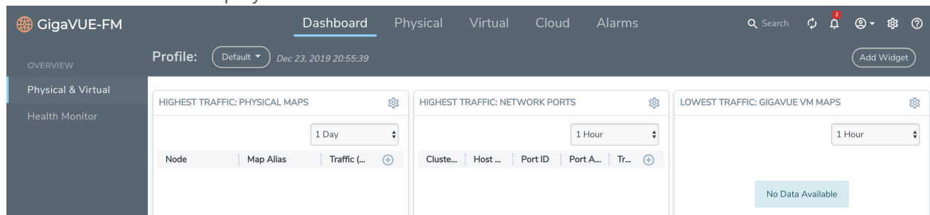
Figure 1 Virtual Dashboard
